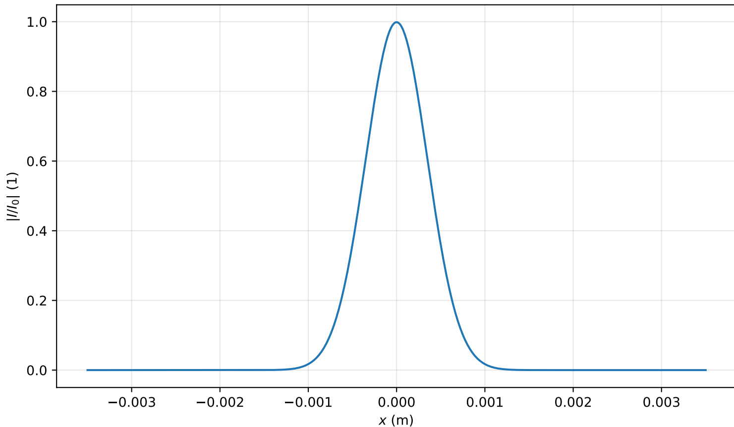
Intensity profile I(x, y = 0, z = 0.159m)/I_0 , P_{in}=0.2P_{cr} , artificial time
